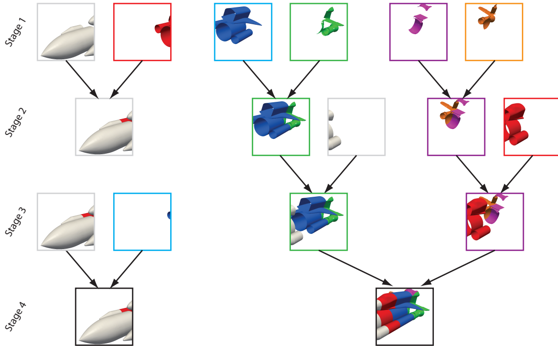
Figure 5.7. Composite network for virtual trees strategy. Arrows represent the passing of data from one state to the next. Processes receiving multiple images composite them together.
